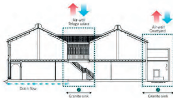
Figure 13. A cross-section diagram showing the flow of water into the house, through the granite air well, and out to the common drain. Source: Gwynn Jenkins and Tan Yeow Woi, Introduction to Heritage Building Materials .
